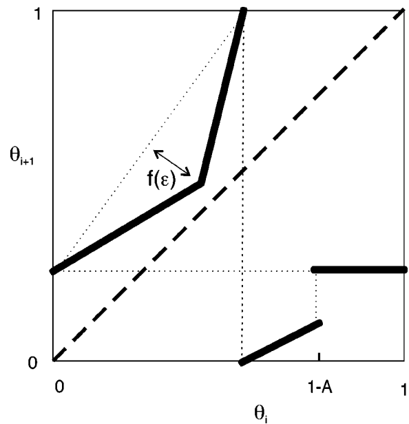
FIG. 3. The graph of a typical g map. The heavy lines are the graph of g , the dashed lines indicate alignments, and the heavy dashed line is the graph of the diagonal line \theta_{i+1} = \theta_i . The function f(\varepsilon) indicates that the amount of kink in the graph depends on \varepsilon , with no kink for \varepsilon = 0 , and a maximum kink when \varepsilon = 1 that causes the elbow to just touch the dashed diagonal line. The kink is exaggerated for clarity, as in practice RSA is rarely higher than 25% ( \varepsilon \leq 0.25 ).
