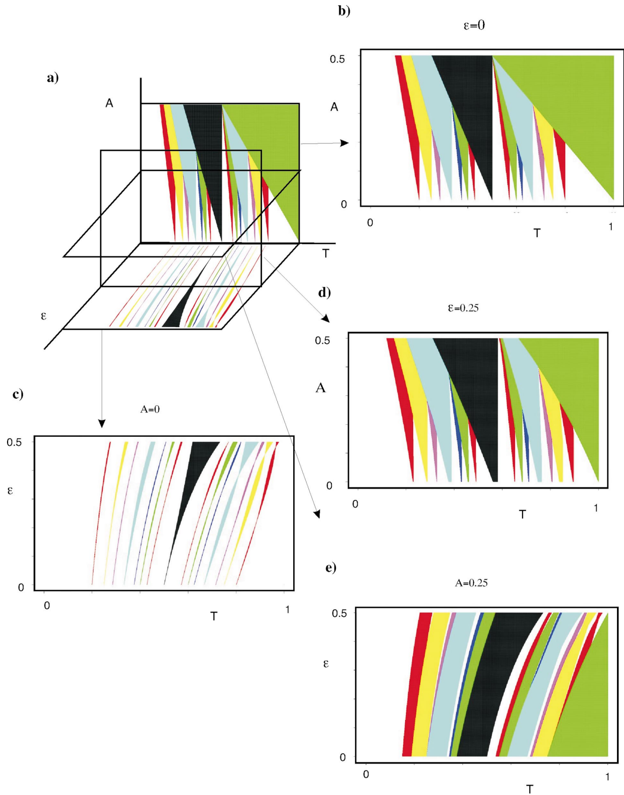
FIG. 4. (Color) Arnold tongues or sausages for our three-parameter circle map. We have determined numerically the phase-locking regions up to depth 4 in a Farey series (i.e., for ratios of breathing to heart-rate of 1/5, 1/4, 2/7, 1/3, 3/8, 2/5, 3/7, 1/2, 4/7, 3/5, 5/8, 2/3, 5/7, 3/4, 4/5 ) and colored each region. In (a) is a 3D representation of the slices used, which are displayed flat in (b)–(e). The slices with \epsilon=0 (b) and A=0 (c) have been seen before (Refs. 2 and 15), and the slices with \epsilon=0.25 (d) and A=0.25 (e) are new, and represent the combined effects of RSA and CVC, but are rather simple modifications or combinations of the previous slices.
