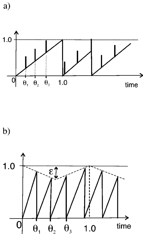
FIG. 1. Integrate-and-fire models. (a) A model (Ref. 12) for the times of inspiration. When the ramping demand for ventilation, augmented by the cardiac spikes that model the influence of heart-beats on respiration (CVC), reaches the dashed threshold line, a new inspiration is begun, and the demand is reset to zero again. RSA is incorporated by using the integrate-and-fire model illustrated in (b) to determine the timing of the cardiac spikes ( \Theta_i ) in (a). In this way, the model combines both RSA and CVC. (b) A model for heart-beat times that includes the effects of RSA. A ramping demand for a heart-beat rises with slope 1/T until it meets the dashed threshold line, when the heart beats, and the demand resets to zero. RSA is modeled by lowering the threshold at the half-way point by an amount \epsilon so that heart-beats increase in frequency during inspiration, and decrease in frequency during expiration. Time is normalized on respiration period, and the period of heart-beats in the absence of RSA is given by the value of T .
