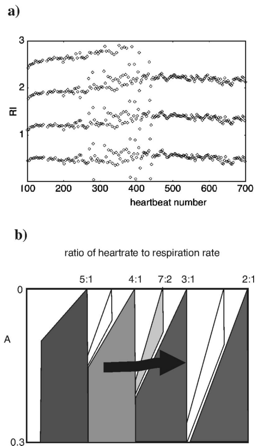
FIG. 2. Plots of RI intervals, and phase-locking regions, from Galletly and Larsen (Ref. 12). The RI interval is the time in seconds between a heart-beat and the next inspiration, as measured in vivo , and in (a) there is a transition from 4:1 locking (in the range 100–250 heart-beats) through 7:2 (in range 250–400 heart-beats) to 3:1 locking. These data were taken at a time when the anesthetized patient's average heart-rate was decreasing steadily while respiration rate remained relatively steady. In (b) is shown schematically (and rather approximately) a corresponding portion of the phase-locking regions determined by repeatedly numerically solving the integrate-and-fire model of Fig. 1(a) using an application called LabView (Ref. 12), and thereby directly determining the phase-locking that is observed for various ratios of heart-rate to underlying respiration rate, and for various values of cardiac spike amplitude A . The heavy arrow that crosses the tongues in (b) is consistent with the sequence of transitions seen in (a) and with the patient's decreasing heart-rate. RSA was set to zero for these calculations. Note that the horizontal axis corresponds to 1/T . Also note the similarity of (b) to Arnold's original plots (Ref. 2).
